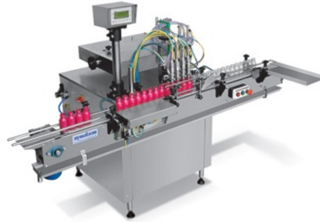
LD 54 PAL Likit Dolum Makinesi Liquid Filling Machine
